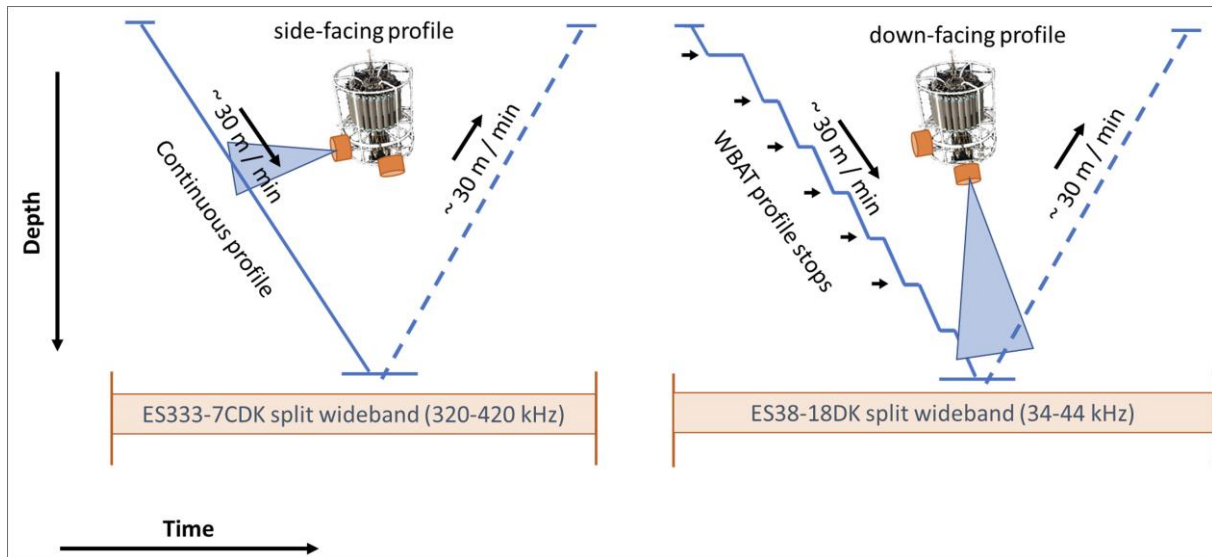
Figure 12: The two CTD WBAT deployment configurations (38 and 333 kHz). Data collection was primarily focused on the downcast, as upcasts (heaving) resulted in some bubble artefacts and occasional stops to fire Niskin bottles for water collection.
