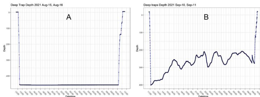
Figure 27: Difference in the effect of ice drift / water currents between two trap lines deployed on different dates as shown by Star Oddi TD probe depth measurements. The indicated depth is the depth of the lower end of the trap line. (A) Hardly any effect. (B) Strong effect.
