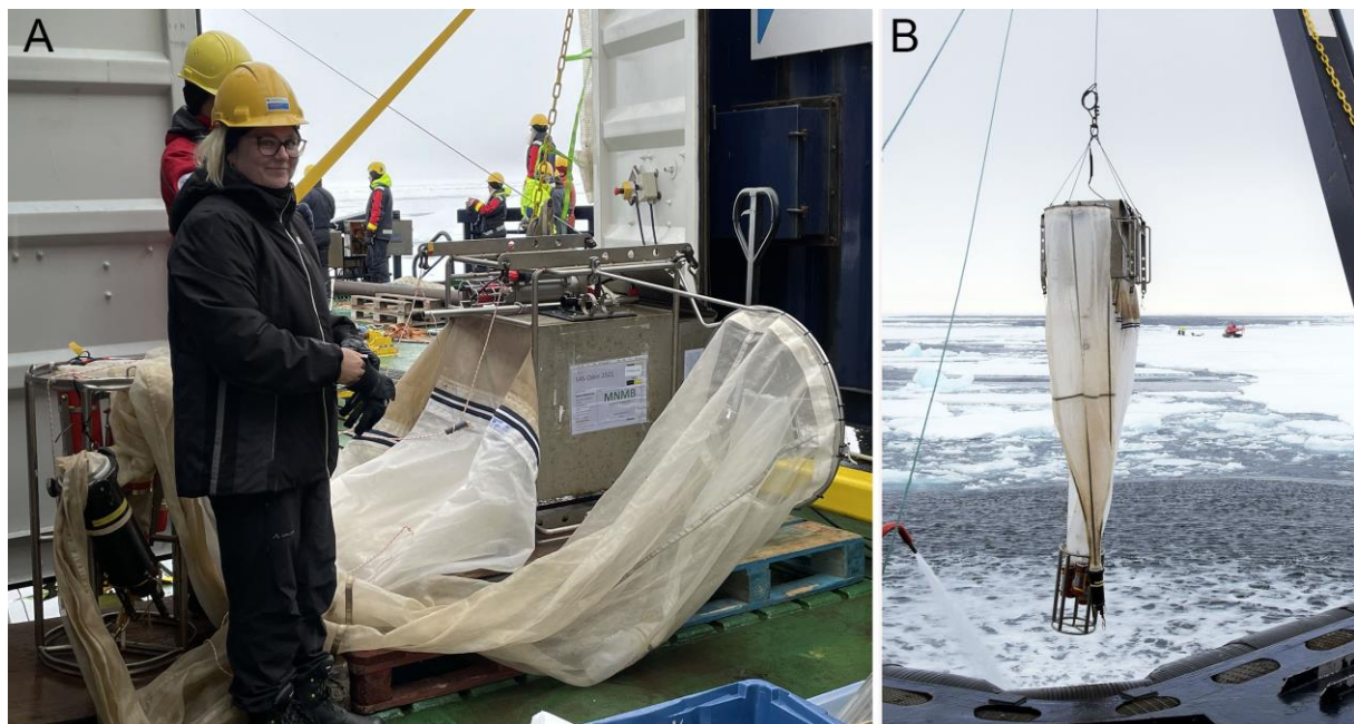
Figure 40: Multinet deployment during the SAS-Oden expedition. (A) Preparations. (B) The net is winched into the water – the water hose is used to keep the ice open. (A) © Pauline Snoeijls-Leijonmalm, (B) © Hans-Jørgen Hansen
