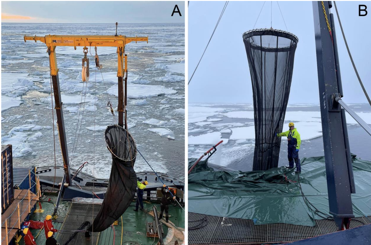
Figure 38: The MIK ring net. (A) Overview of the aft deck before deployment of the MIK net. (B) The weights are launched and the MIK net is stretched downward in the water (A) © Pauline Snoeijs-Leijonmalm, (B) © Nicole Hildebrandt
