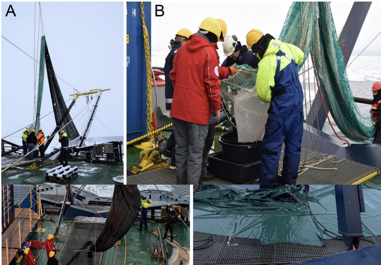
Figure 37: Emptying the cod-end of the beam net. (A) Overview of the aft deck after retrieval of the beam net. (B) Collecting the catch. (A,B) © Hans-Jørgen Hansen
